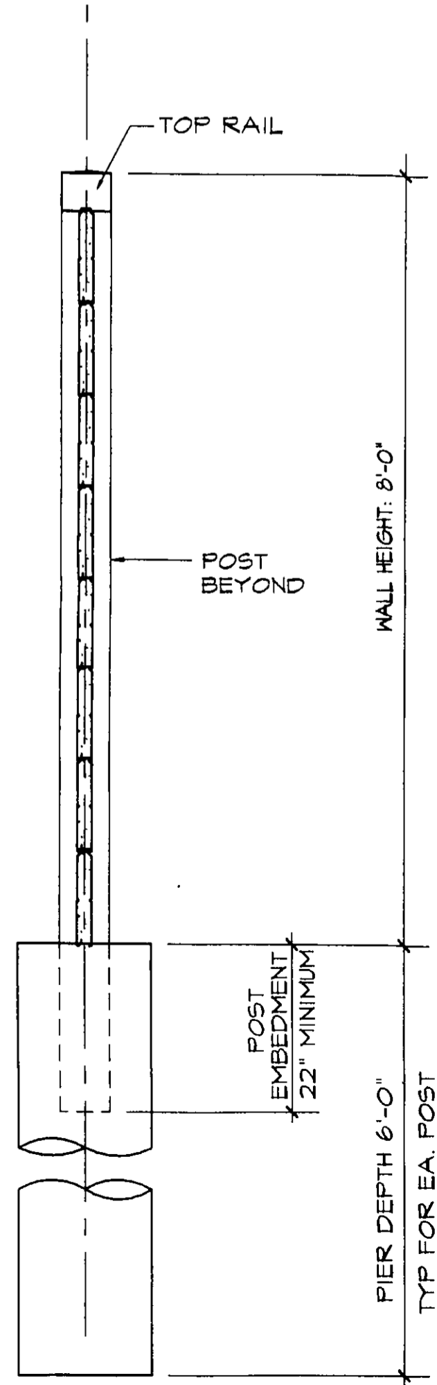
SECTION-TOP RAIL SCALE: 2" = 1'-0"
