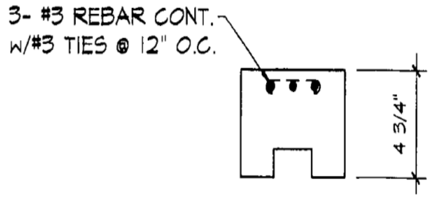
SECTION-TOP RAIL SCALE: 2" = 1'-0"
