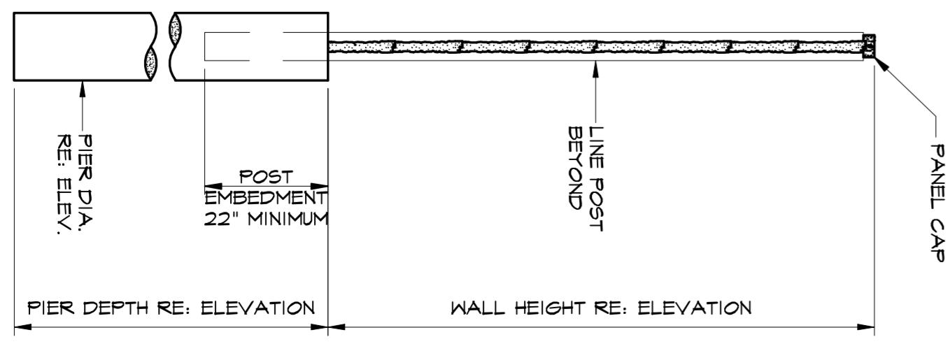
SECTION - SCREENING WALL SCALE 1/2" = 1'-0"
